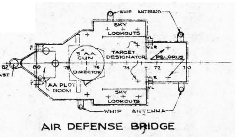
AIR DEFENSE BRIDGE
