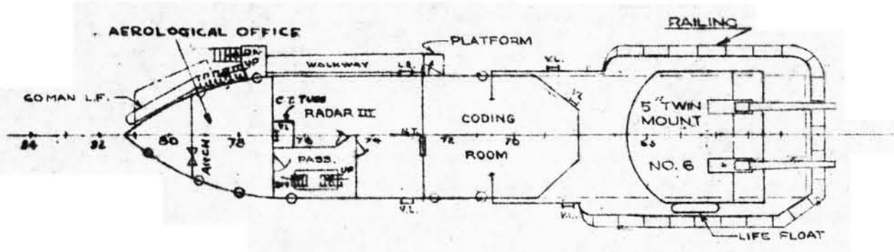
AEROLOGICAL PLATFORM
