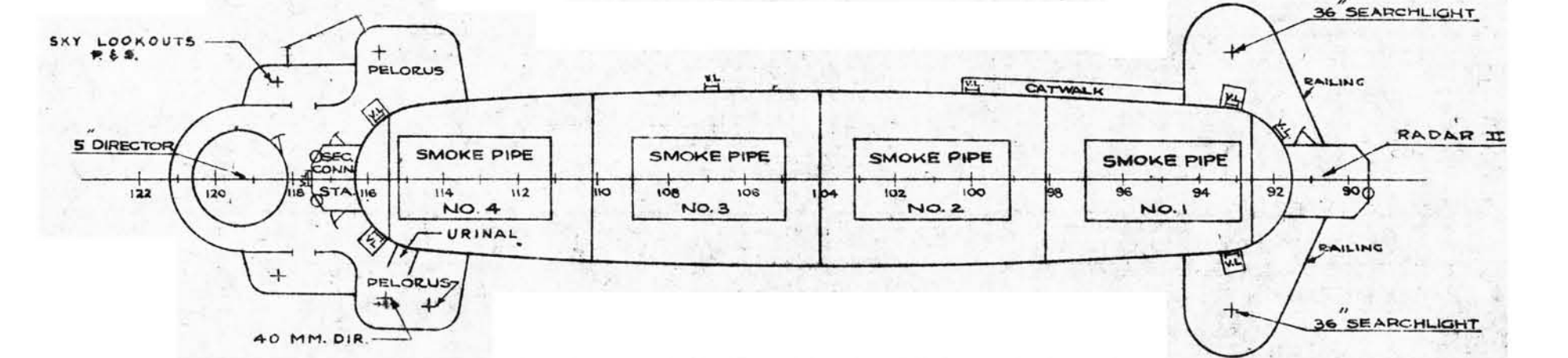
DIRECTOR & SEARCHLIGHT PLATFORM
